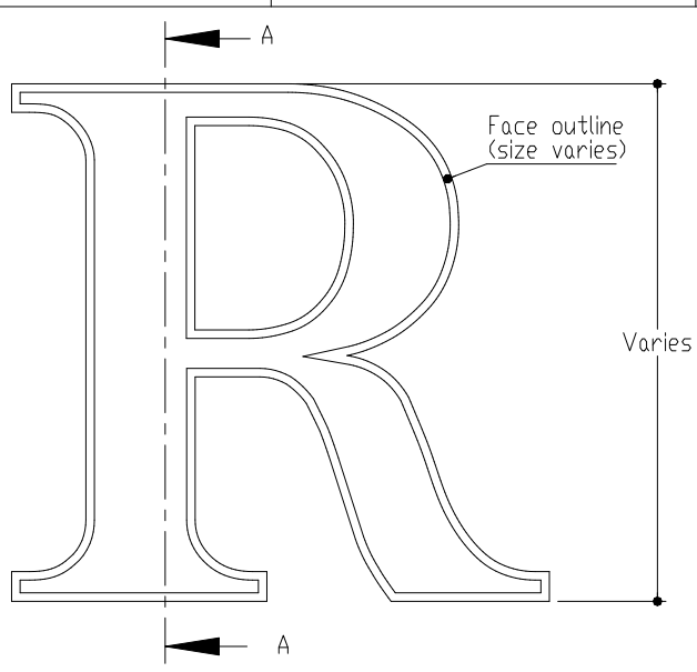
FRONT VIEW II SCALE 1:5
