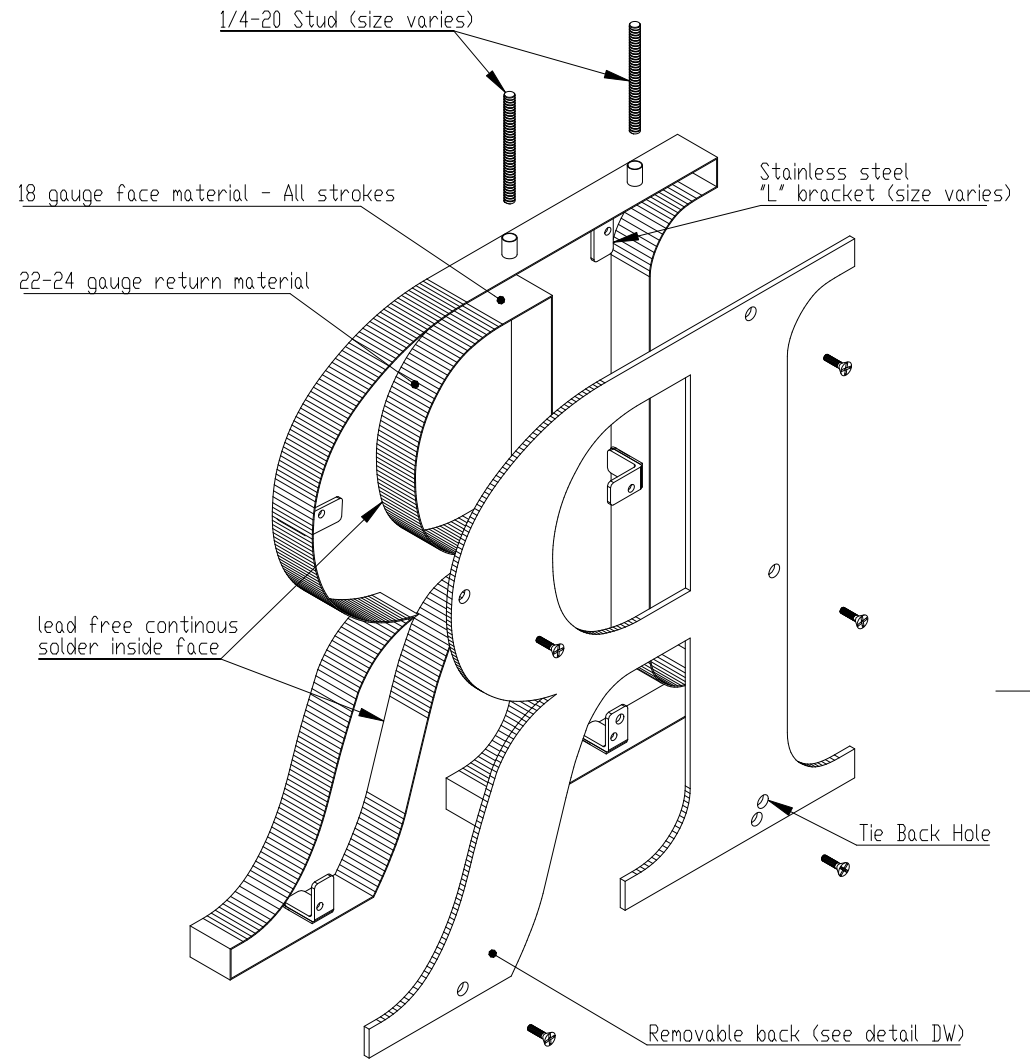
ISOMETRIC BACK VIEW II SCALE 1:3.5
