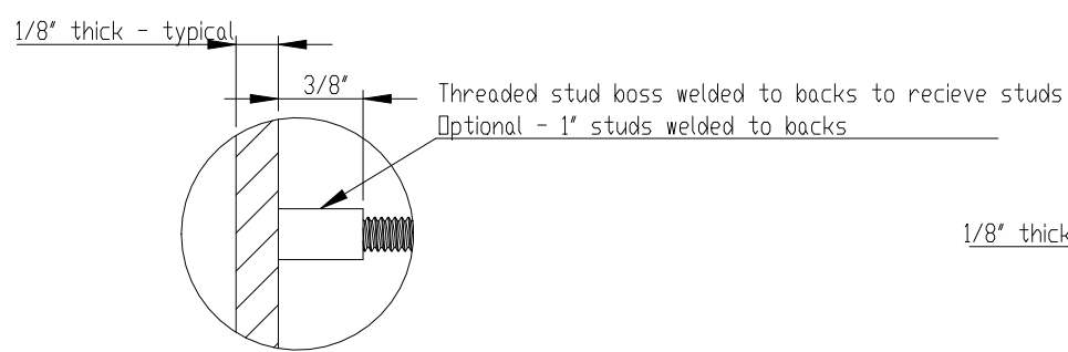
DETAIL DW II SCALE 1 : 1
