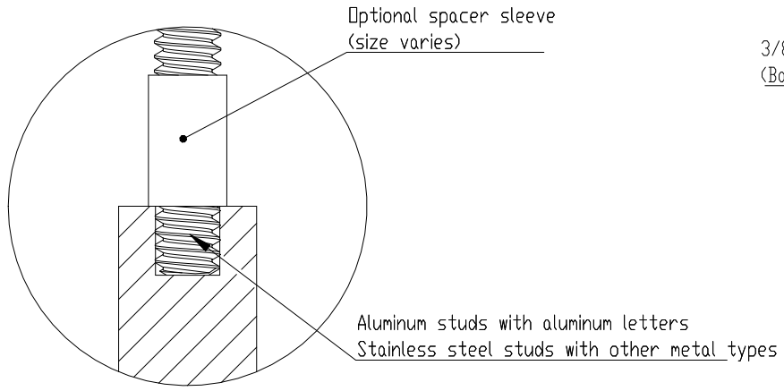
DETAIL DW II SCALE 2:1
