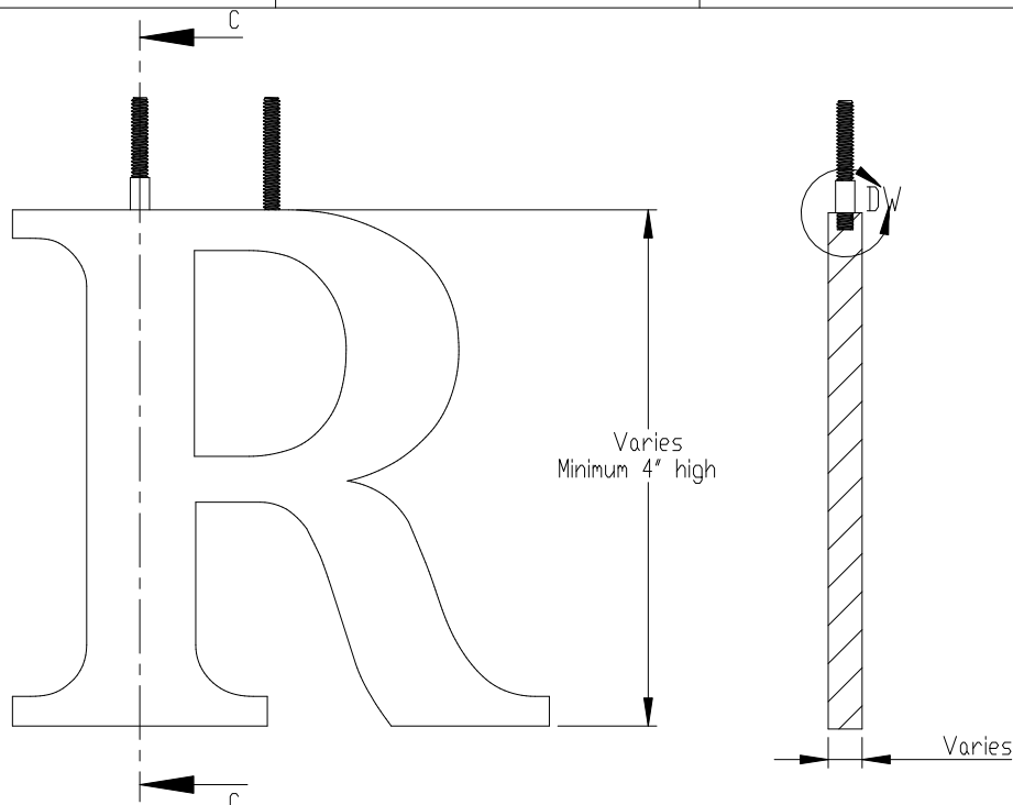
FRONT VIEW II SCALE 1:2.5
