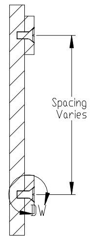
SECTION VIEW A-A II SCALE 1:2.5
