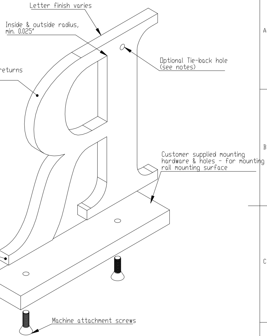
ISOMETRIC BACK VIEW II SCALE 1:1.75
