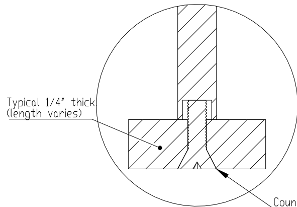
DETAIL DW II SCALE 2:1
