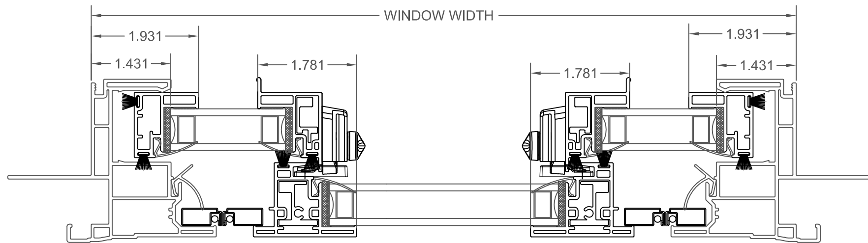
Model 1903 3-Lite Slider 1/4 - 1/2 - 1/4
