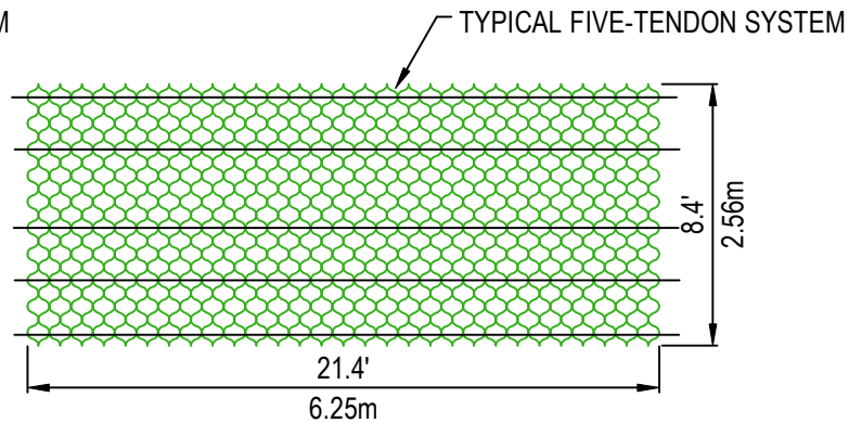
5 TENDON SPACING
