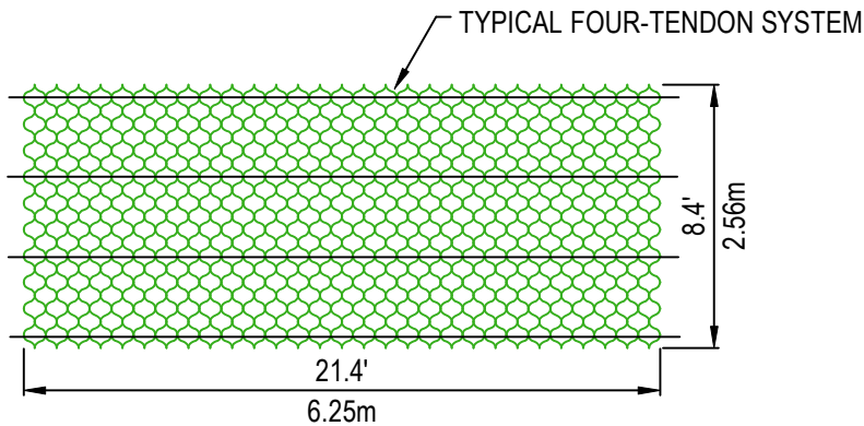
4 TENDON SPACING
