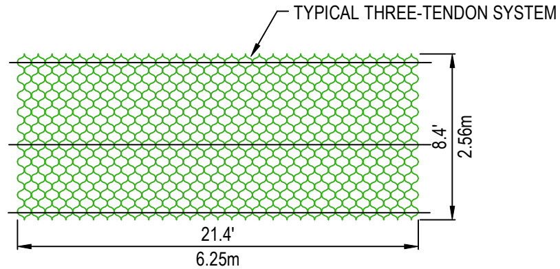
3 TENDON SPACING
