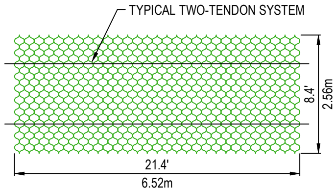
2 TENDON SPACING
