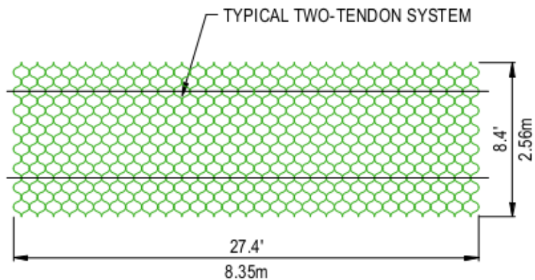
2 TENDON SPACING
