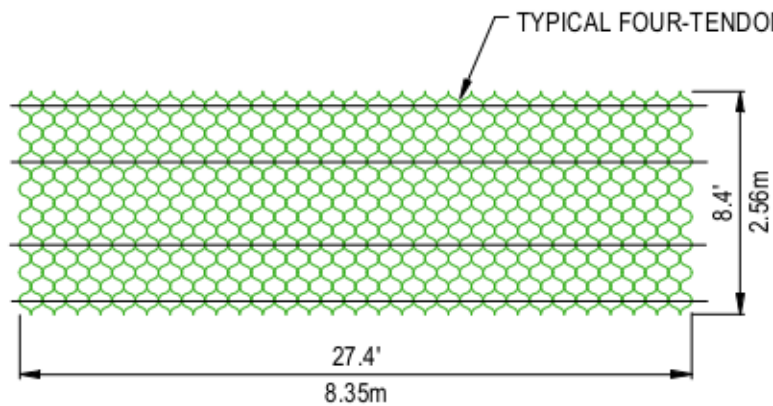
4 TENDON SPACING
