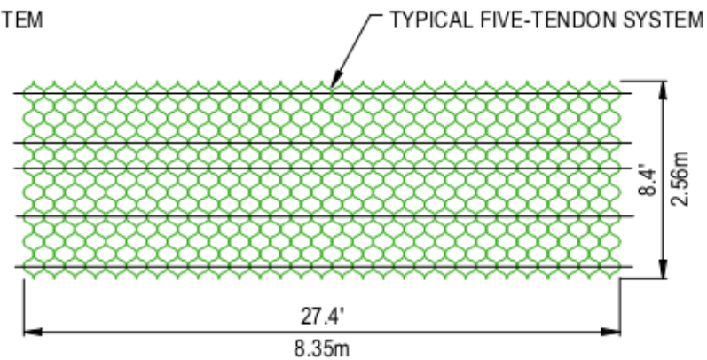
5 TENDON SPACING
