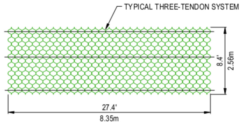
3 TENDON SPACING
