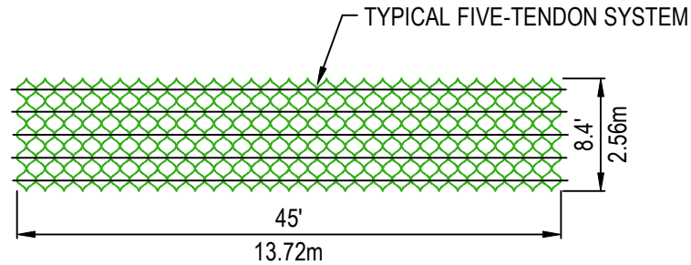
5 TENDON SPACING
