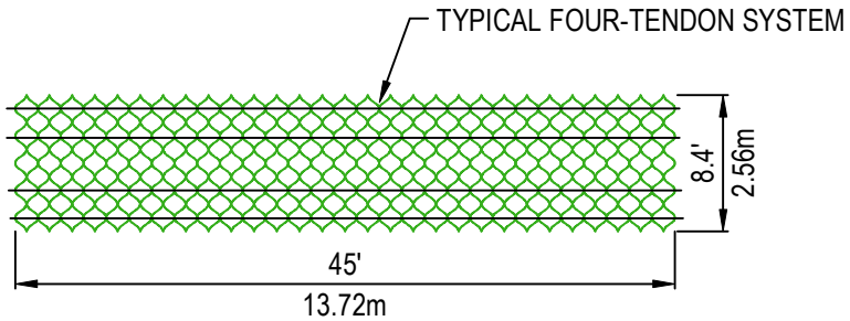
4 TENDON SPACING
