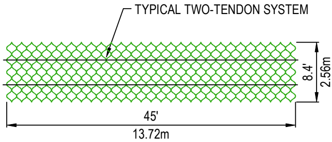
2 TENDON SPACING
