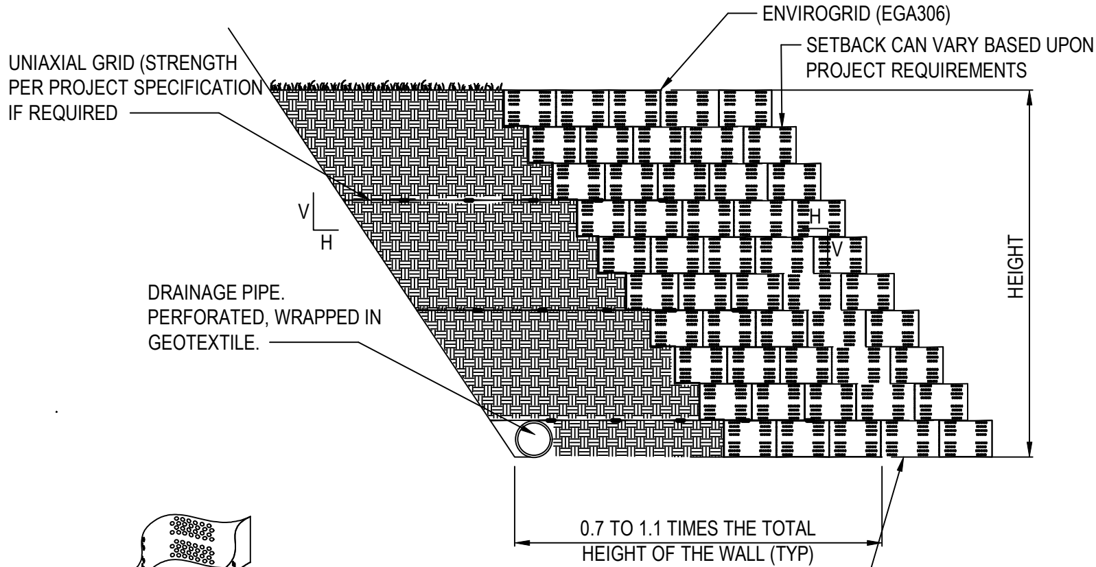
CROSS SECTION
