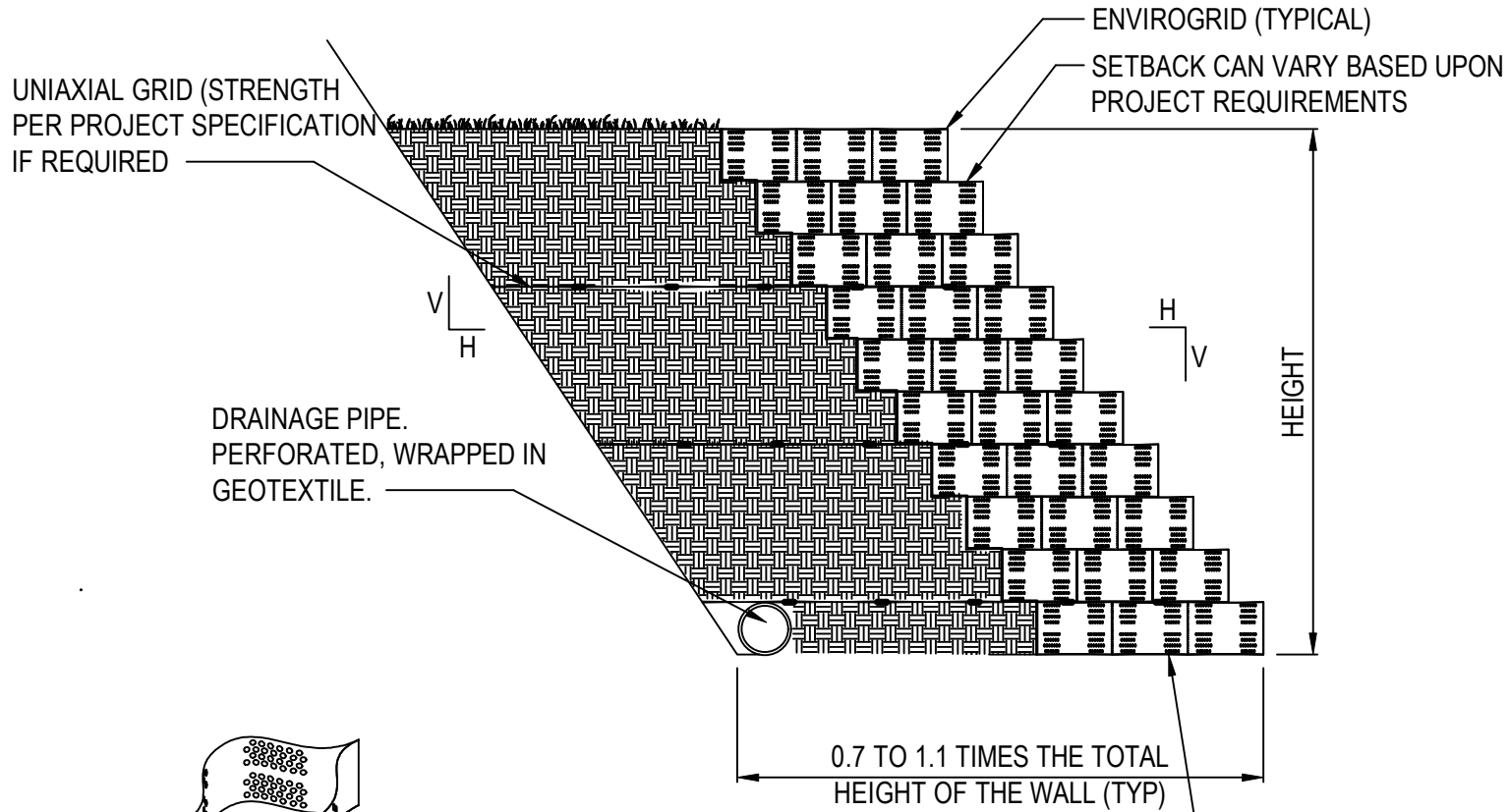
CROSS SECTION
