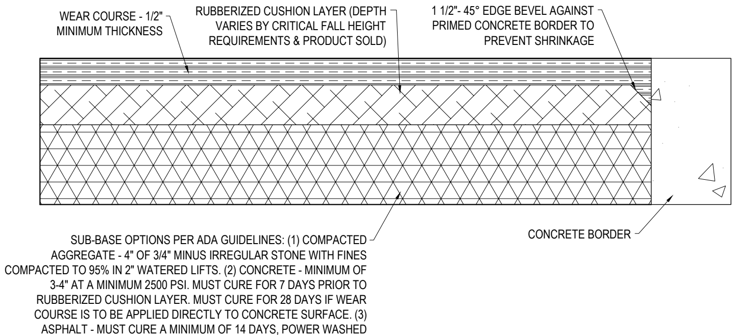
SECTION VIEW
