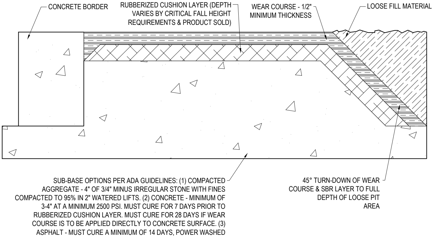
SECTION VIEW
