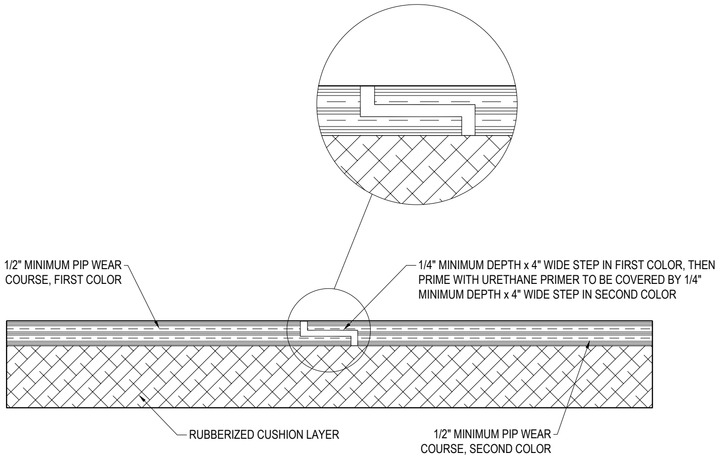
SECTION VIEW
