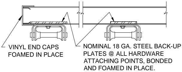
HINGE DETAIL
