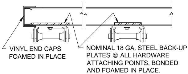
HINGE DETAIL
