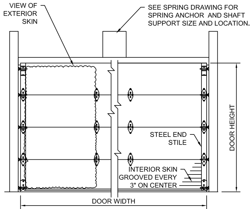
INTERIOR ELEVATION
