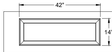
PANEL DIMENSIONS
