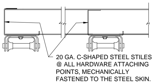
HINGE DETAIL
