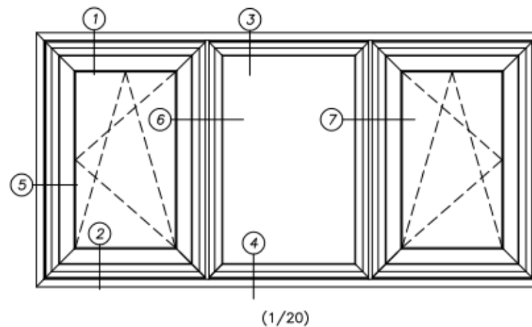
Harvey Building Products N.C. Axio Tilt & Turn Window 3-Wide Factory Mull V/F/V Triple Glaze IG (1/2 Scale)
