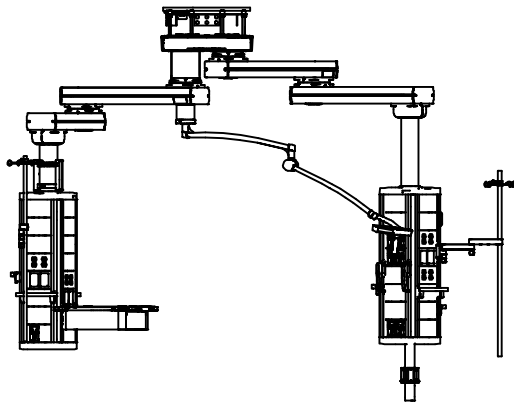
ELEVATION (DUAL)
