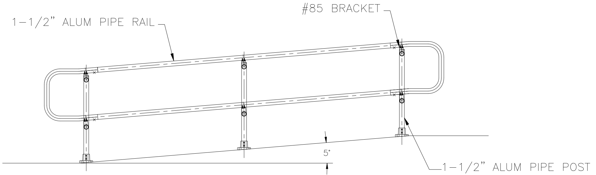
TYPICAL A.D.A. HANDRAIL DETAIL
