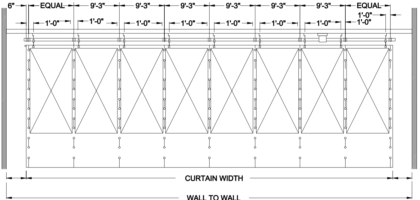
CURTAIN ELEVATION
