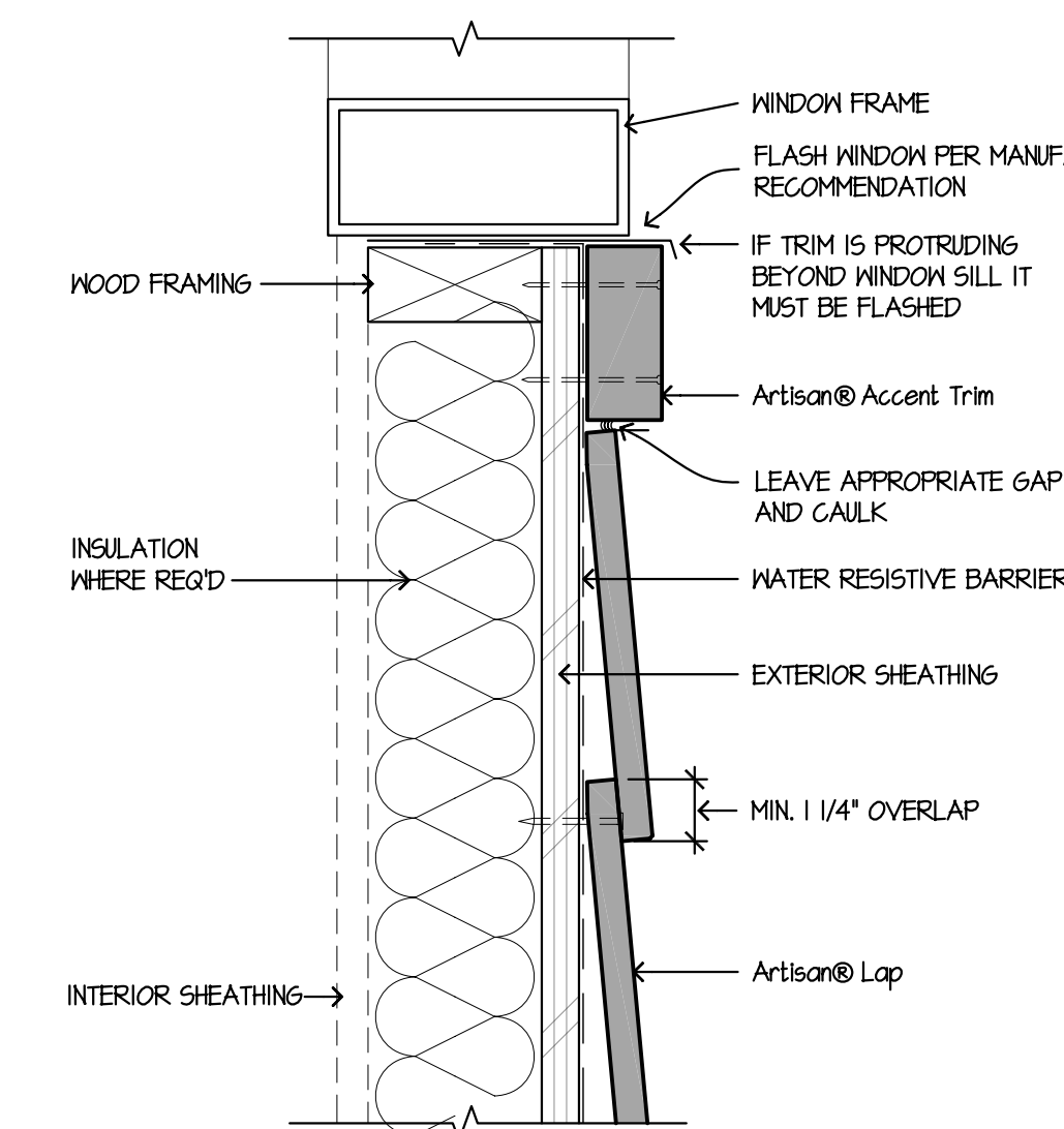
5 HORIZONTAL LAP VIEW SCALE: 3/4"=1'-0"
