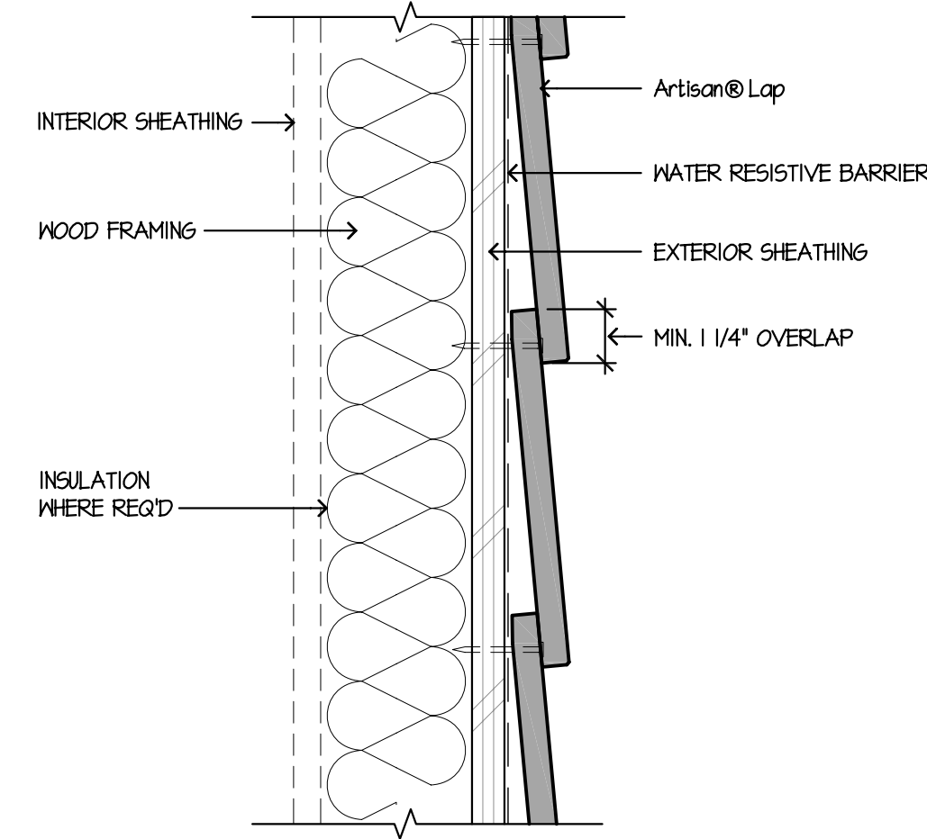
5 HORIZONTAL LAP VIEW SCALE: 3/4"=1'-0"
