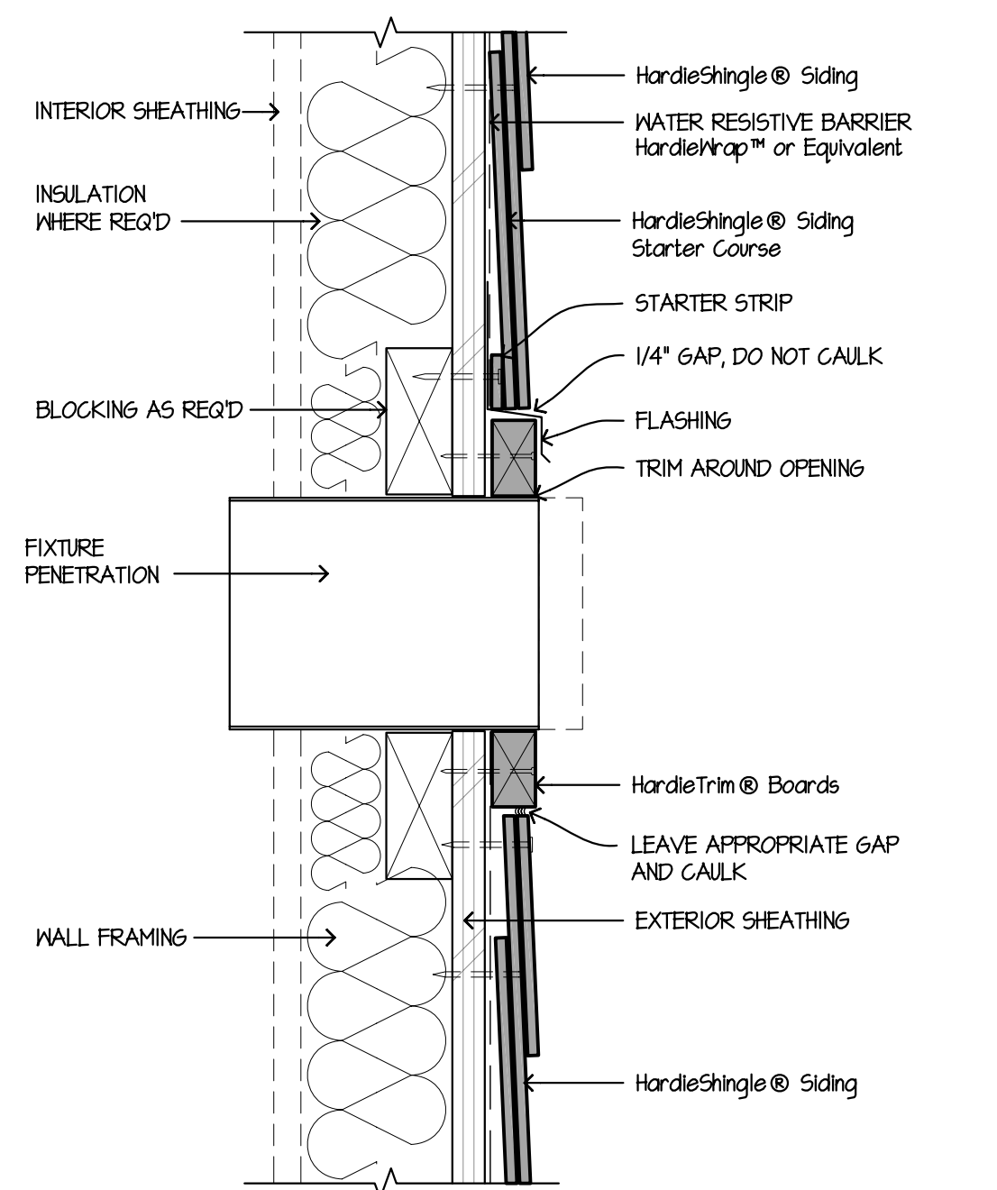
7 FIXTURE PENETRATION SCALE: 3/4"=1'-0"
