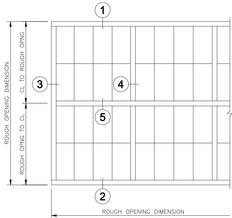
WALL ELEVATION
