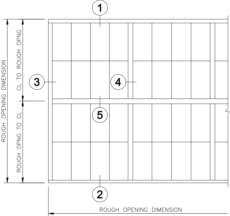
WALL ELEVATION
