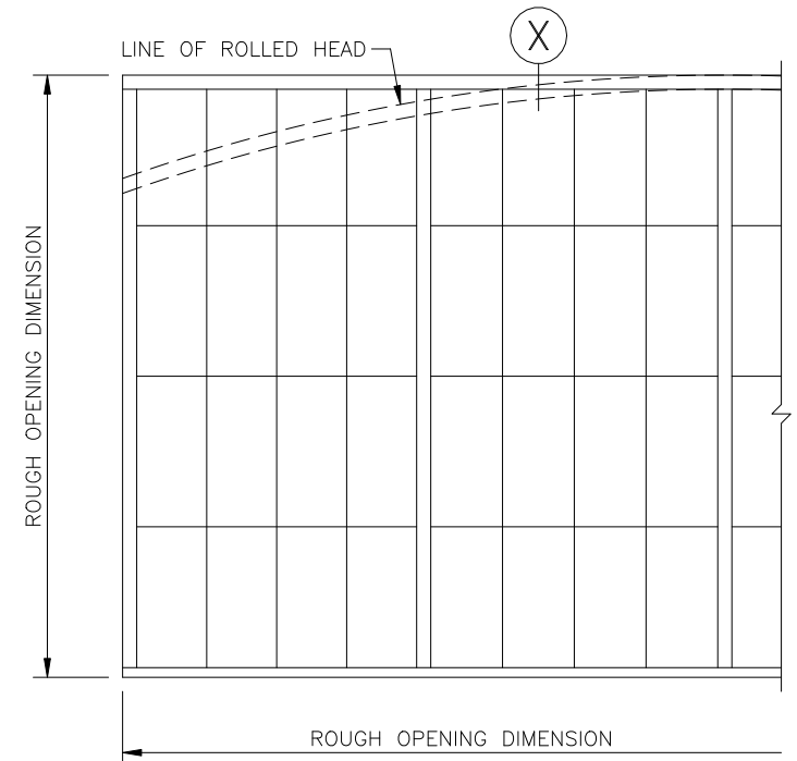
WALL ELEVATION
