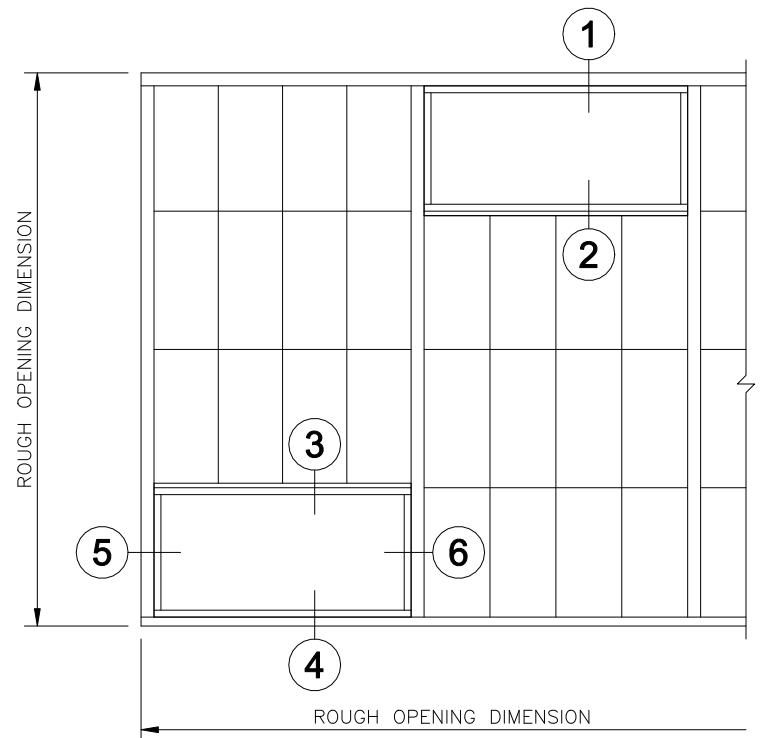
WALL ELEVATION
