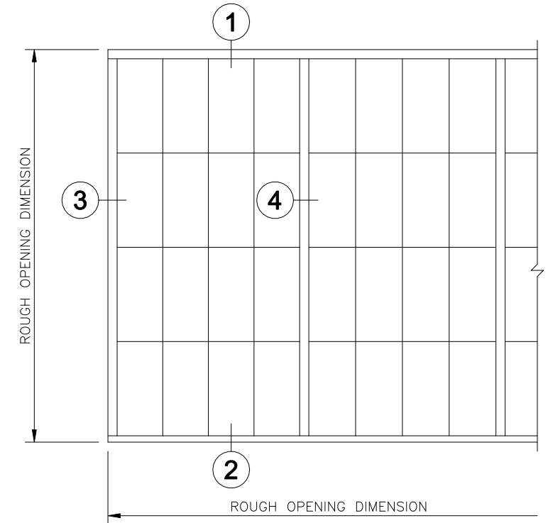
WALL ELEVATION
