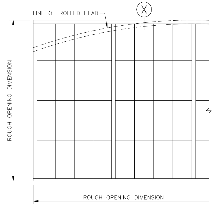
WALL ELEVATION
