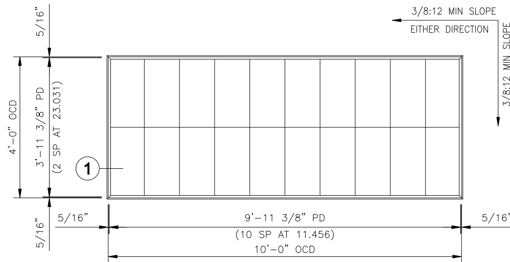
4' x 10' SKYLIGHT S-410-3A
