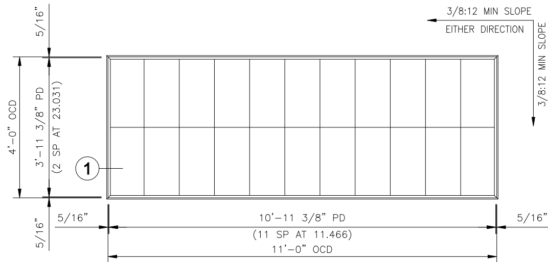
4' x 11' SKYLIGHT S-411-3A
