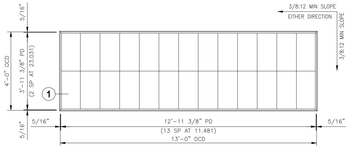
4' x 13' SKYLIGHT S-413-3A
