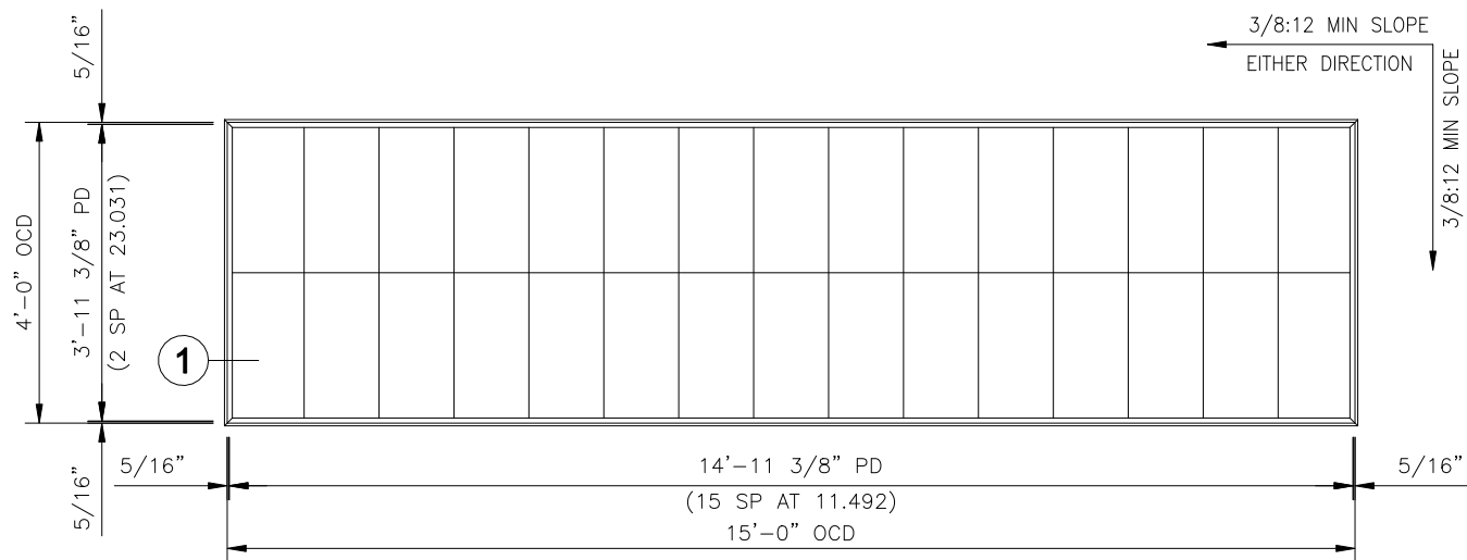
4' x 15' SKYLIGHT S-415-3A
