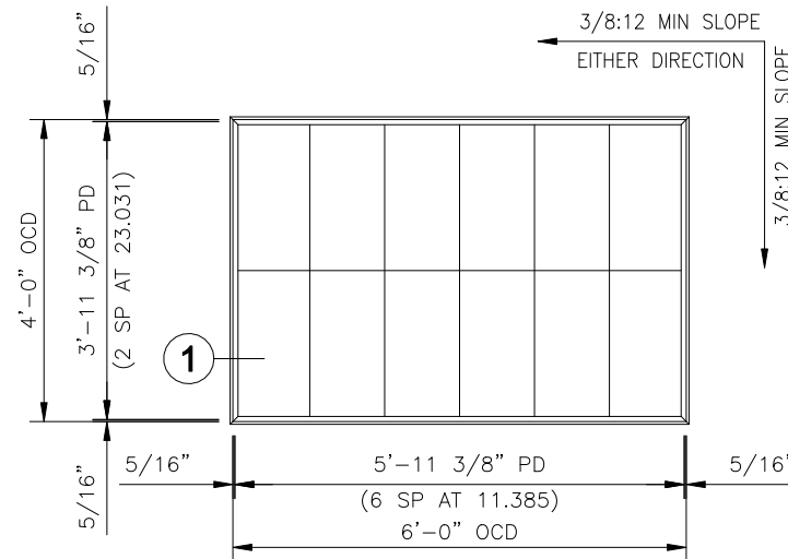
4' x 6' SKYLIGHT S-46-3A
