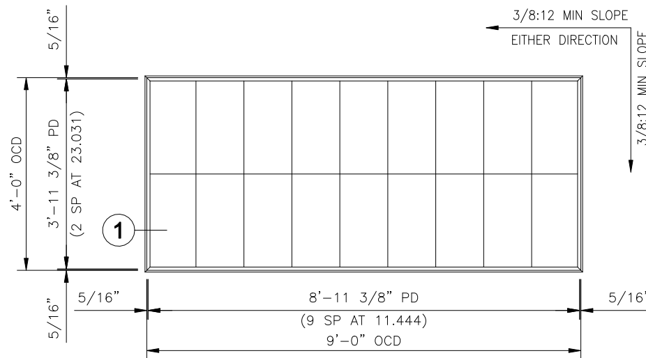
4' x 9' SKYLIGHT S-49-3A
