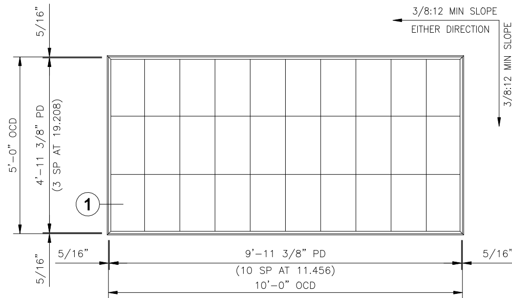
5' x 10' SKYLIGHT S-510-3A
