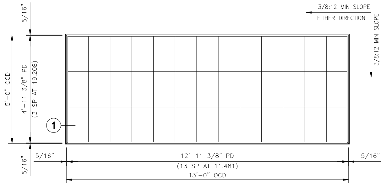
5' x 13' SKYLIGHT S-513-3A
