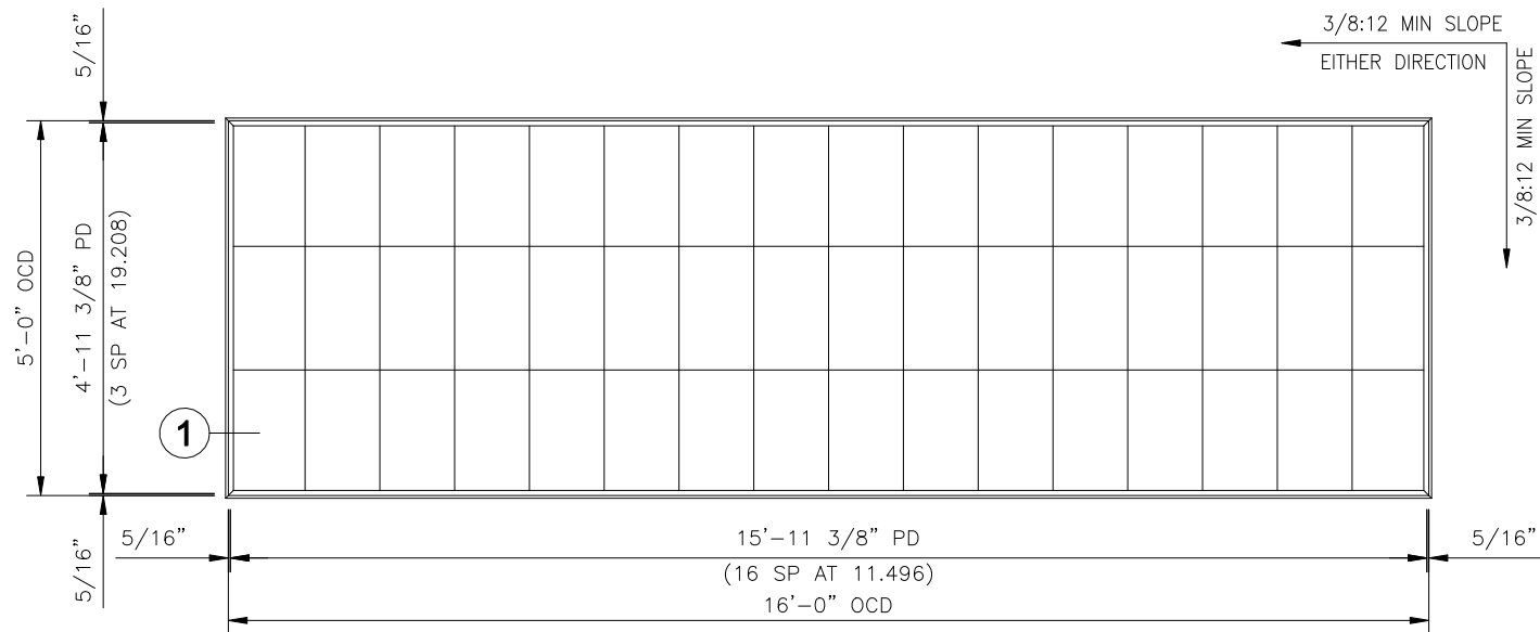
5' x 16' SKYLIGHT S-516-3A
