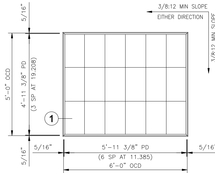
5' x 6' SKYLIGHT S-56-3A
