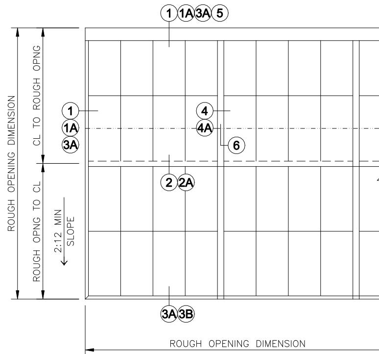
ROOF PLAN
