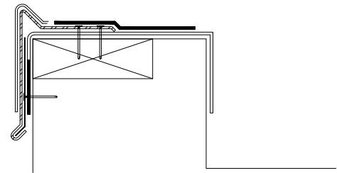
CONDITION #2: (TYPICAL) METAL EDGE AT PARAPET WALL EDGE
