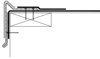
CONDITION #1: (TYPICAL) METAL EDGE AT ROOF EDGE
