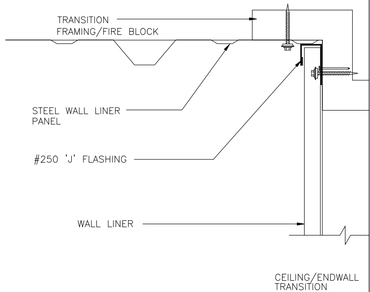
STEEL LINER
