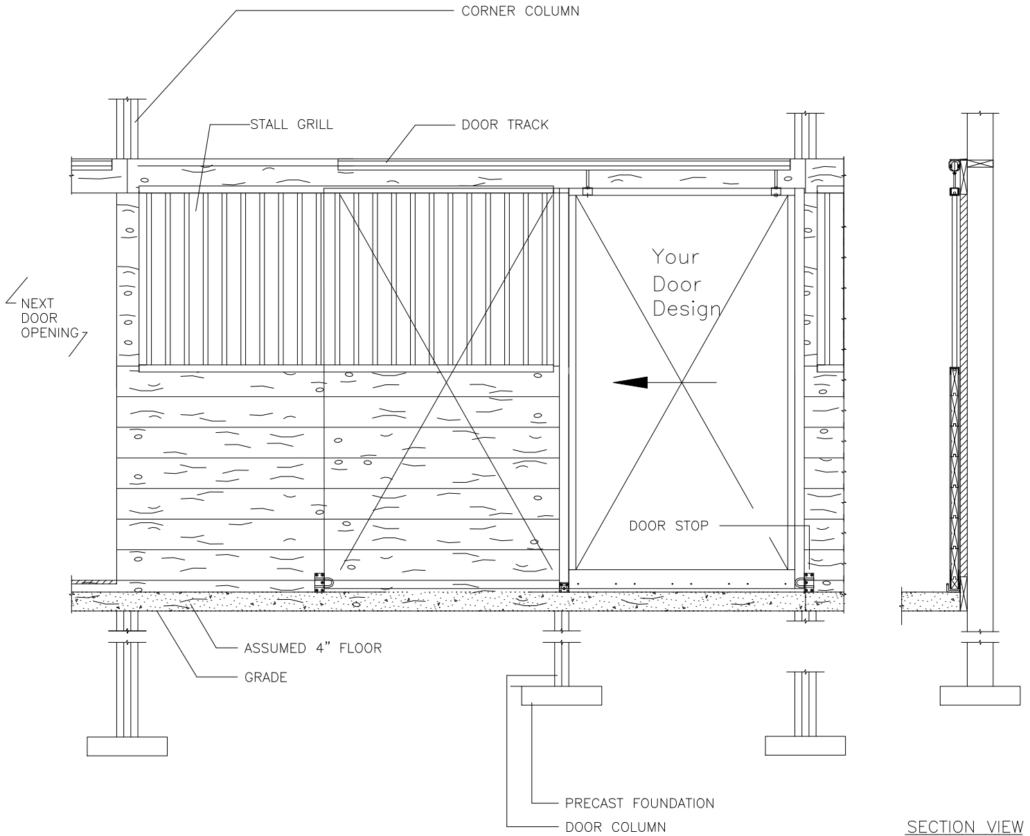
ELEVATION VIEW
