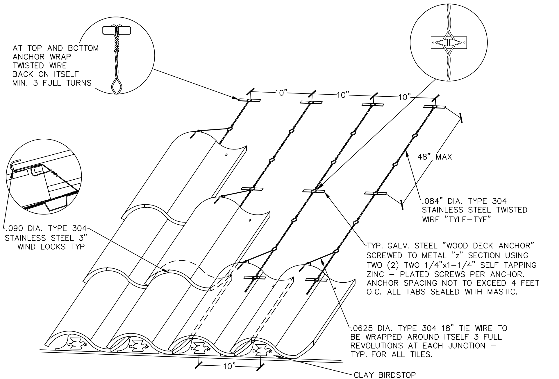
CLASSIC "S" MISSON "TYLE-TYE" FIELD DETAIL (MTL. DECK)
