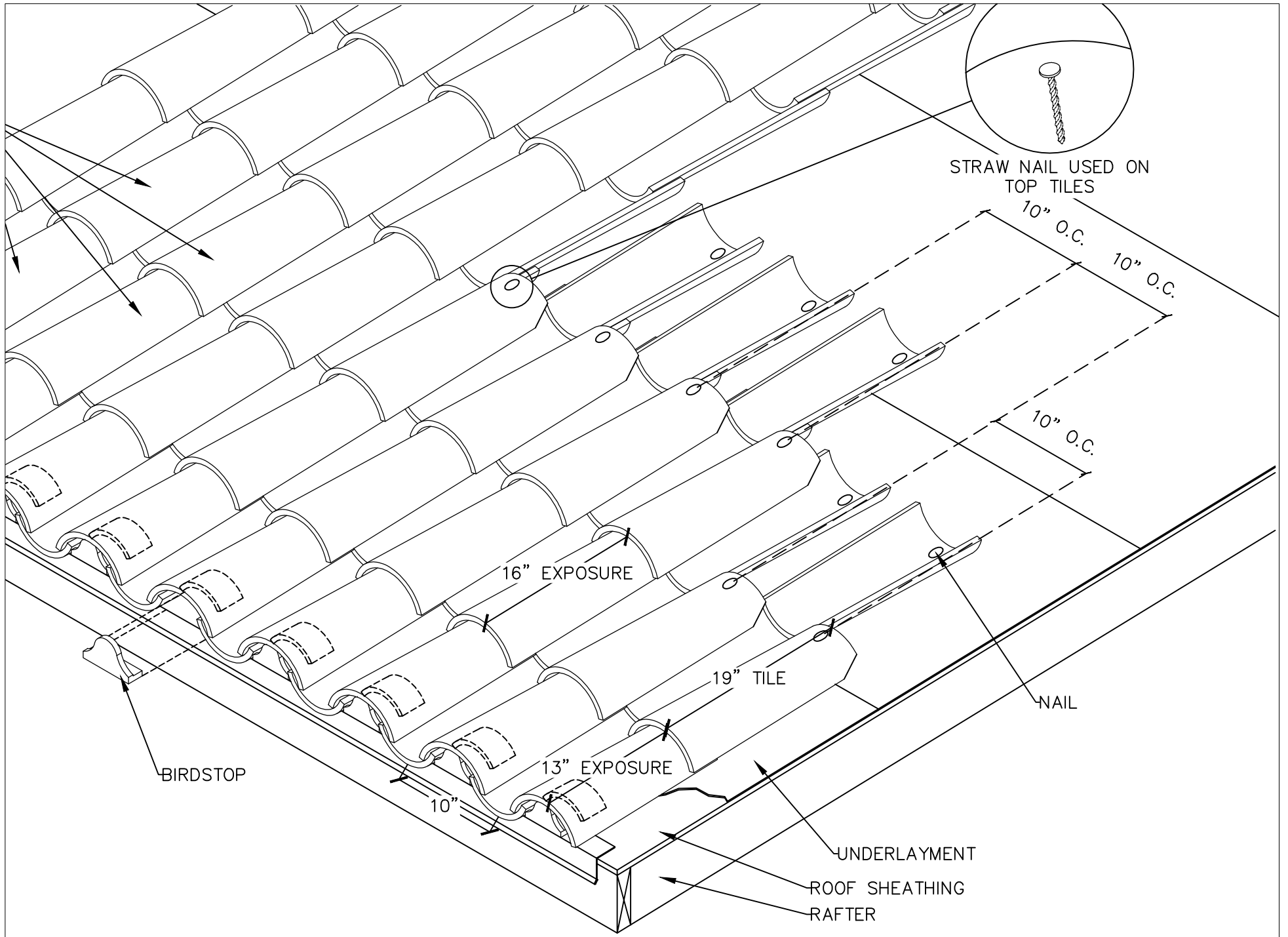
CLASSIC TAPERED MISSION NAIL ON SYSTEM MCA - CLASSIC TAPERED - MTL - 3D N.T.S.
