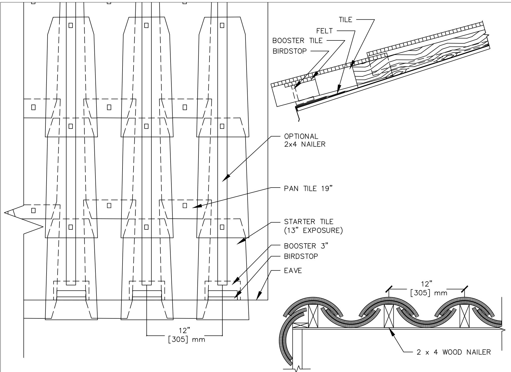
BARREL MISSION NAILER INSTALLATION CORONA TAPERED MISSION
