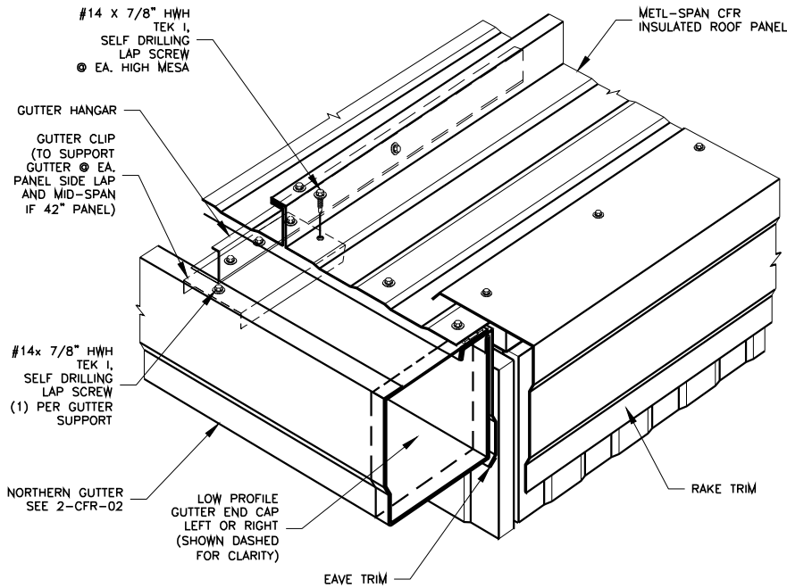
END CAP DETAIL
