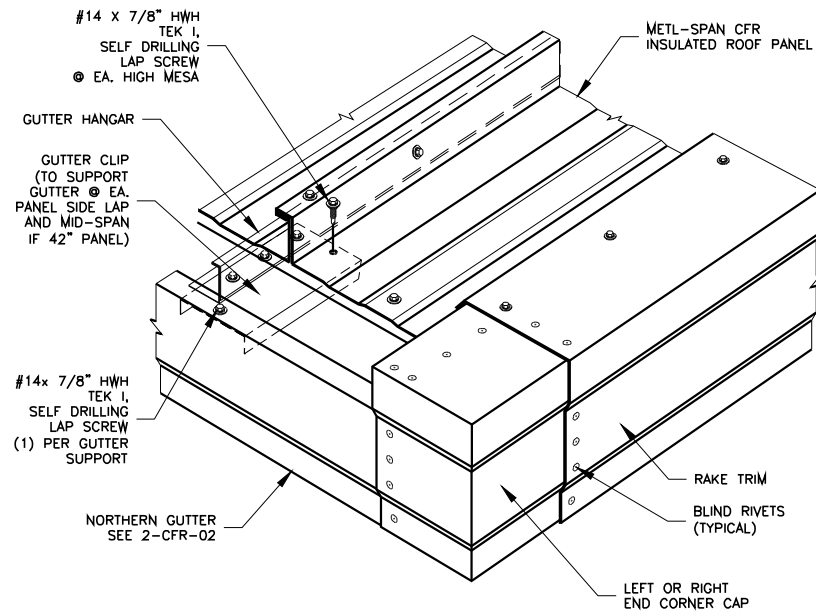
CORNER CAP DETAIL
